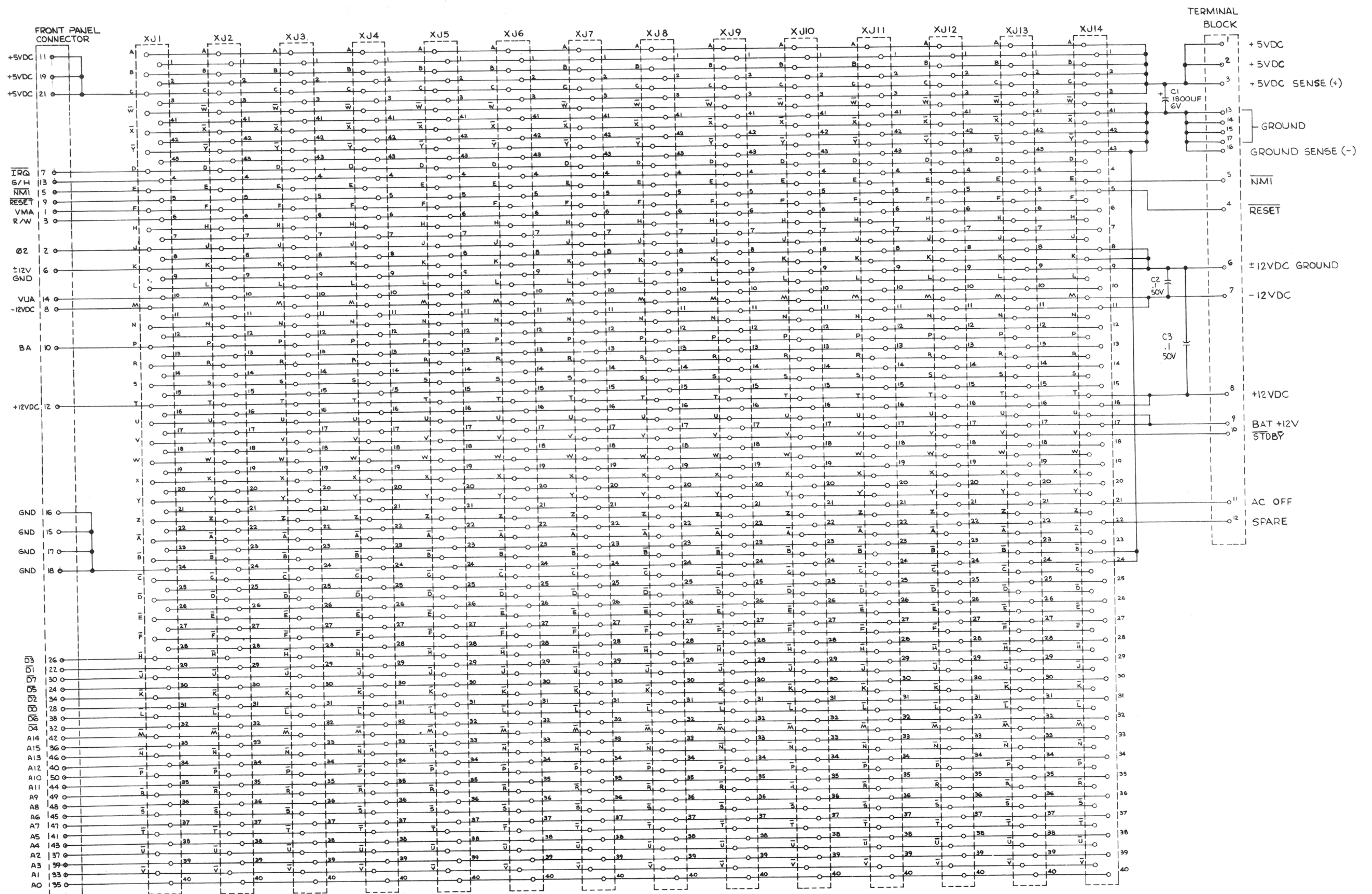
FIGURE 5-8. Motherboard Schematic Diagram
