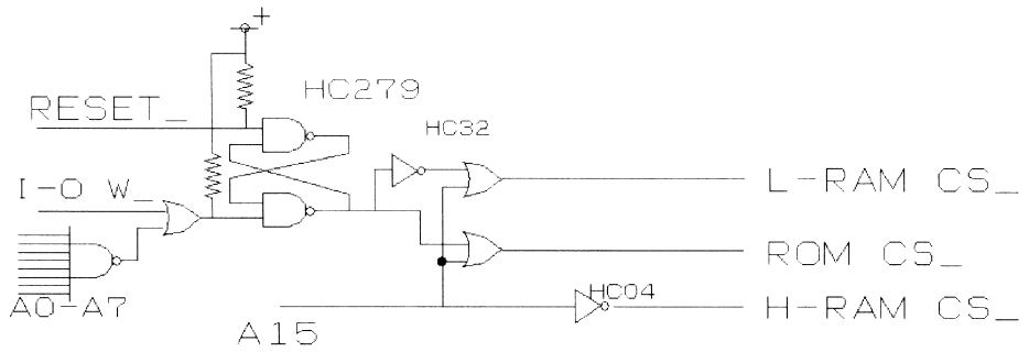
I/O, ROM, RAM CS
